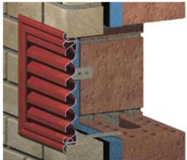
IF38-IW In-Wall
